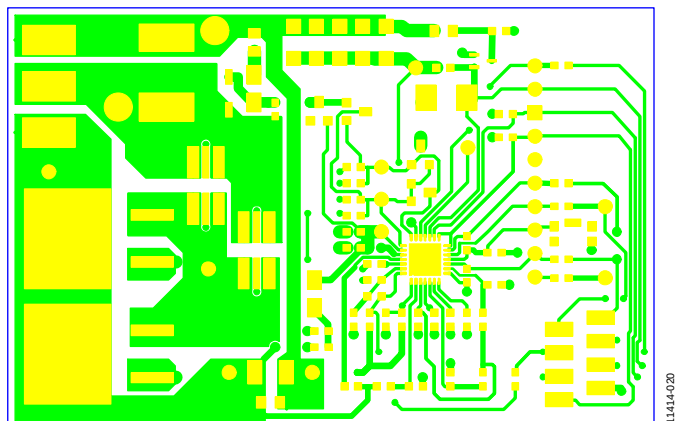
Figure 12. Top Layer
