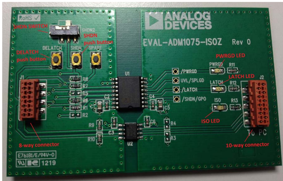
Figure 4. EVAL-ADM1075-ISOZ Board
