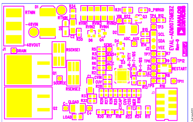
Figure 14. Assembly Top
