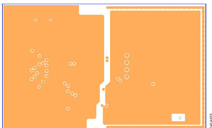
Figure 18. Inner Layer 3
