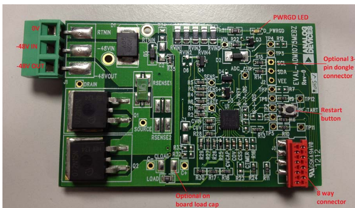
Figure 3. EVAL-ADM1075MEBZ Board
