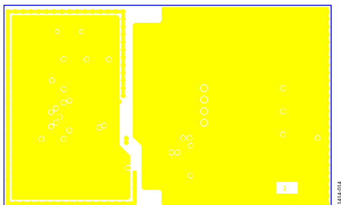
Figure 17. Inner Layer 2
