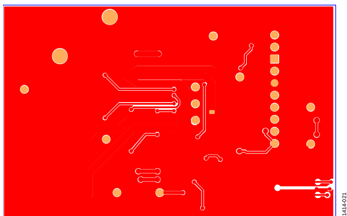
Figure 13. Inner Layer 2
