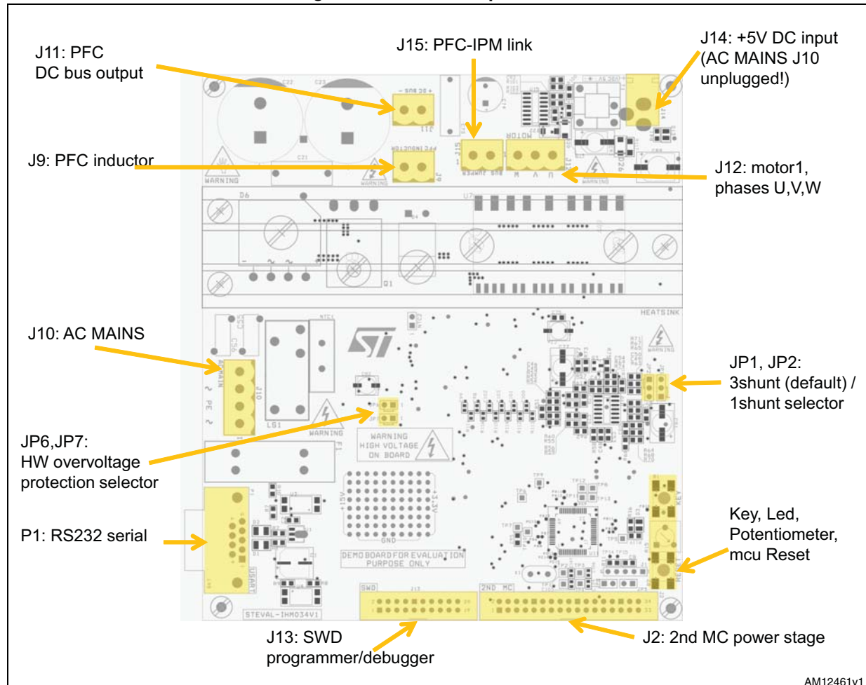
Figure 12. Connector placement
