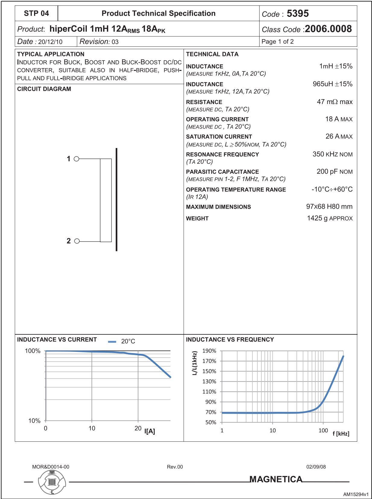
Figure 17. Technical sheet of PFC inductor (page 1 of 2)
