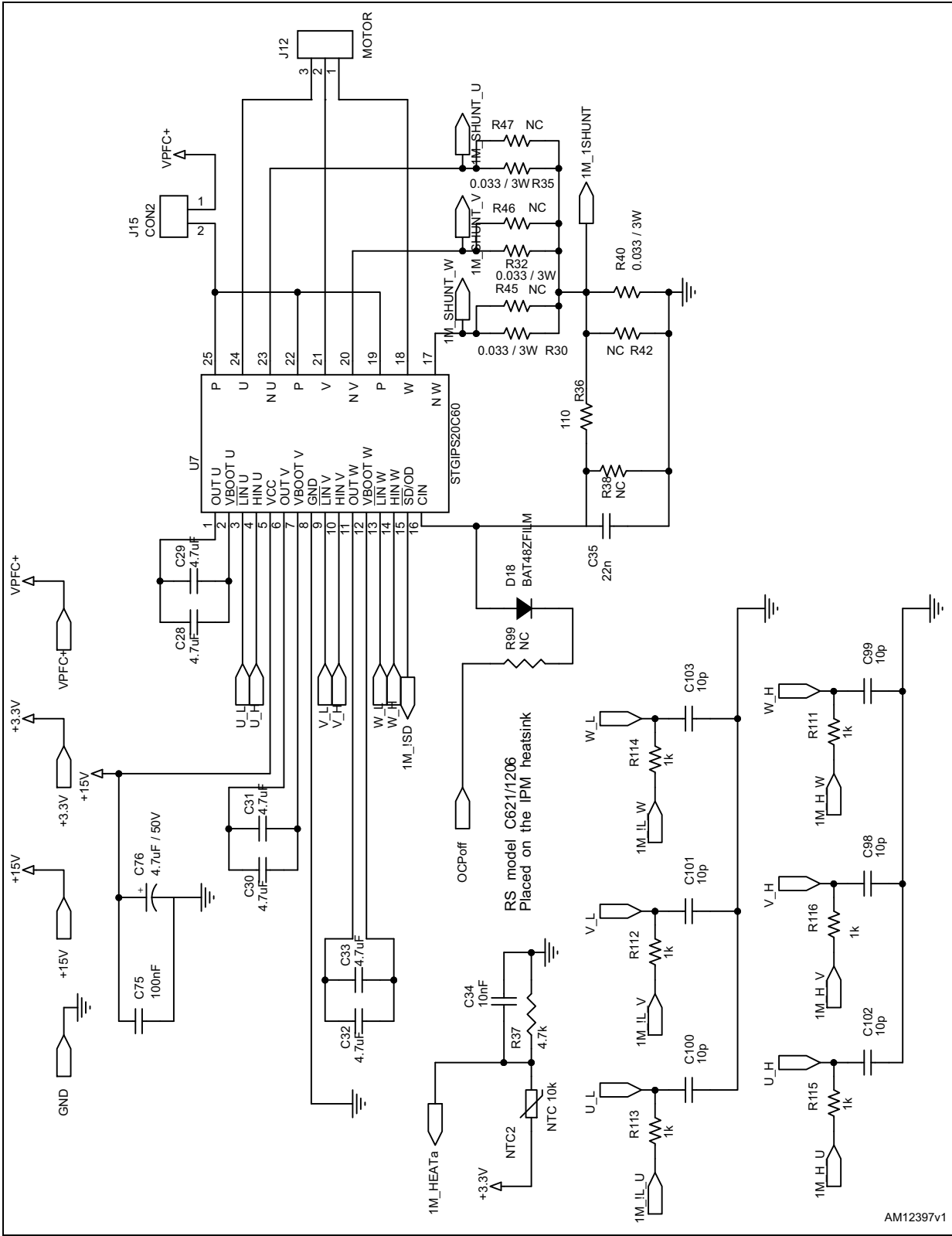
Figure 8. Schematic (6 of 9)
