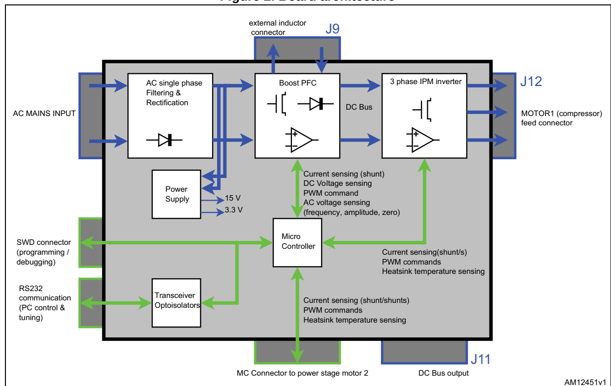
Figure 2. Board architecture
