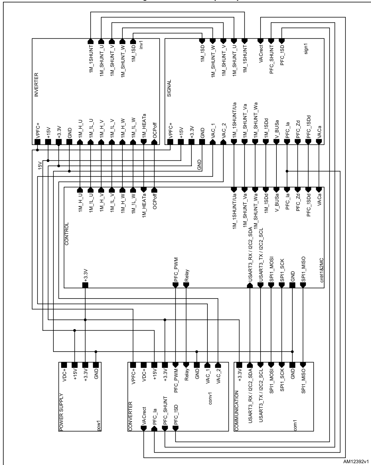
Figure 3. Schematic (1 of 9)
