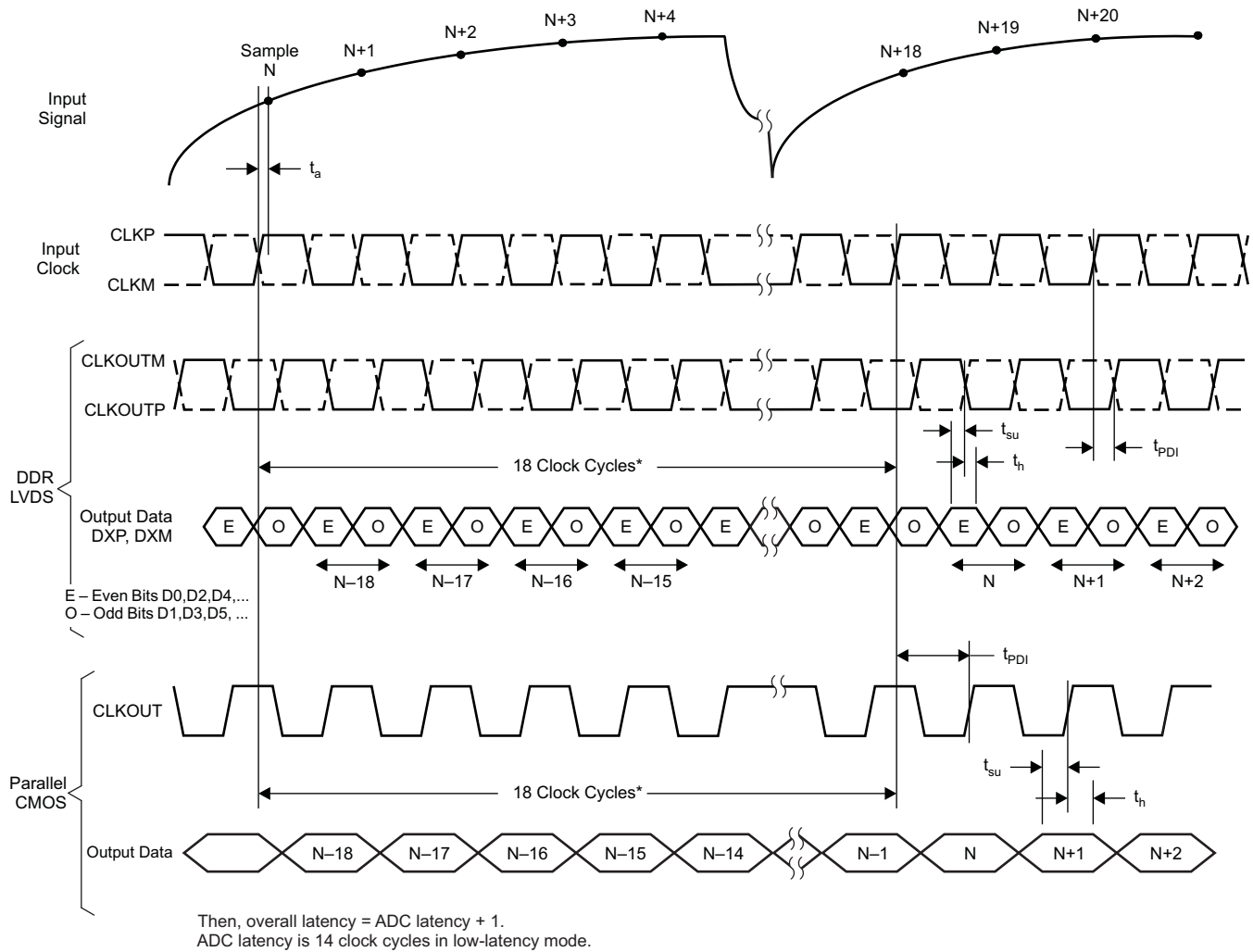
Figure 2. Latency Diagram
