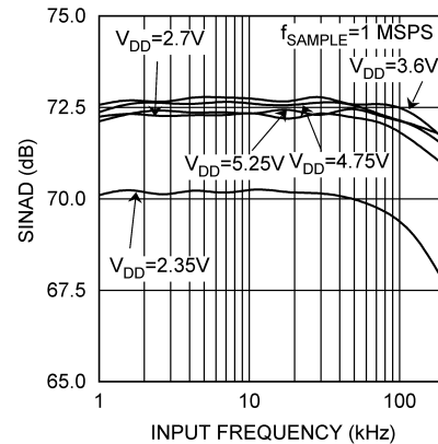
Figure 12. ADCS7476 SINAD vs Input Frequency, 1 MSPS
