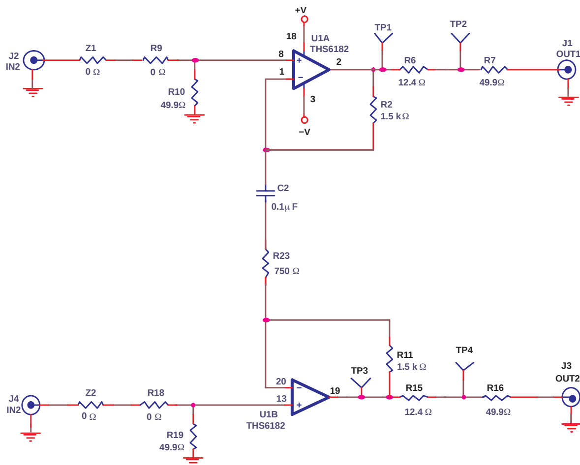
Figure 3–1. Default Configuration Operation
