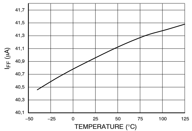
Figure 38. I_{FF} vs. Temperature
