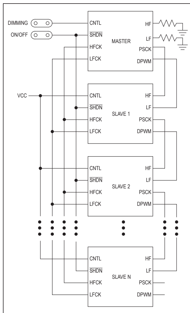
Figure 6. Master-Slave Operation
