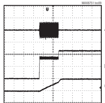
SECONDARY SHORT-CIRCUIT PROTECTOR AND TIMEOUT
