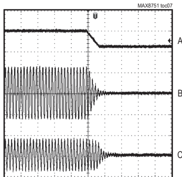
DPWM SOFT-START
