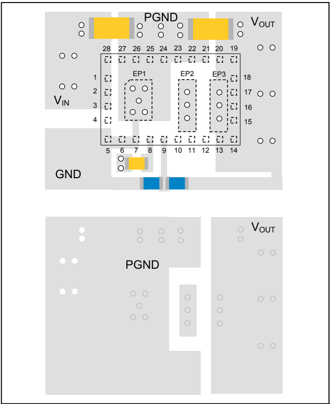
Figure 3. Layout Recommendation
