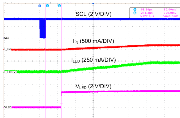
Time (200 \mu\text{s} /DIV) Mode bits (Reg 0x01 bit[1:0]) = 10 (Torch mode)
