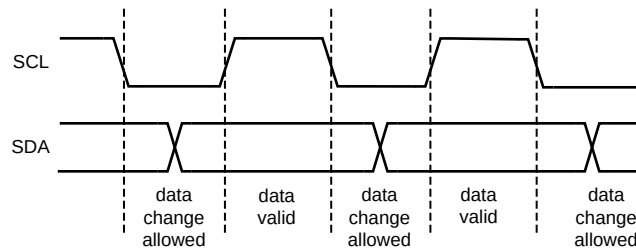
Figure 20. Data Validity Data
