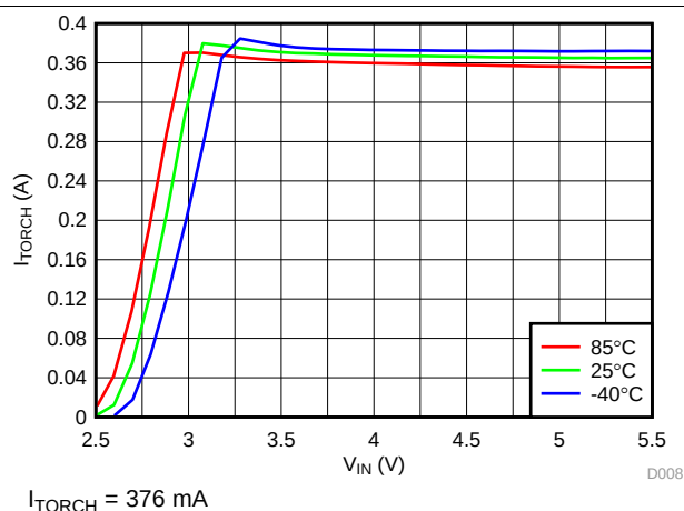
Figure 9. LED Torch Current vs Input Voltage
