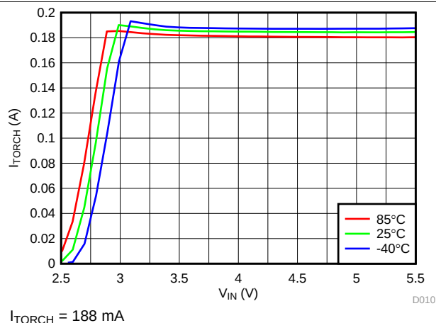
Figure 11. LED Torch Current vs Input Voltage
