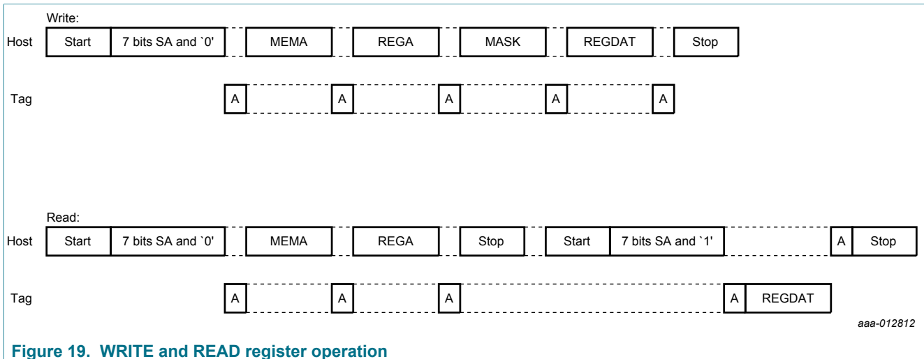
Figure 19. WRITE and READ register operation
