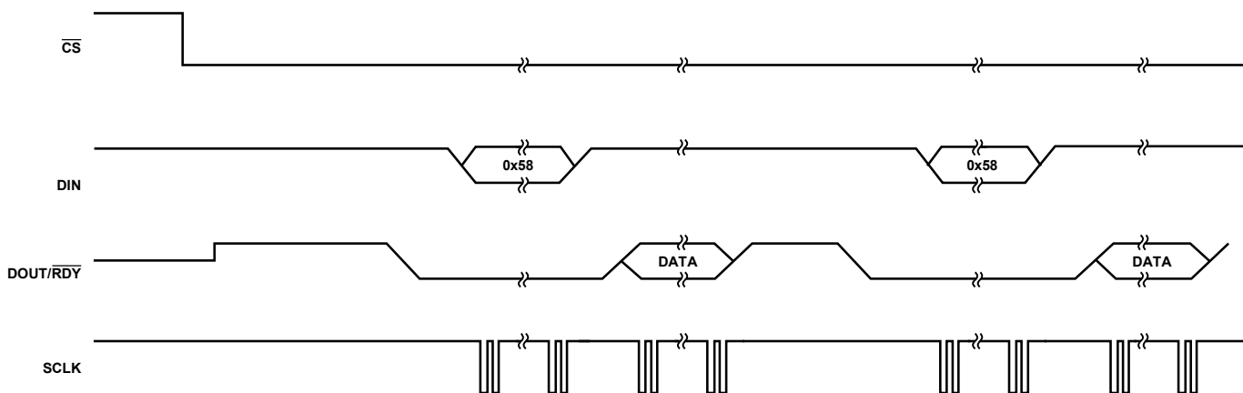
Figure 26. Continuous Conversion
