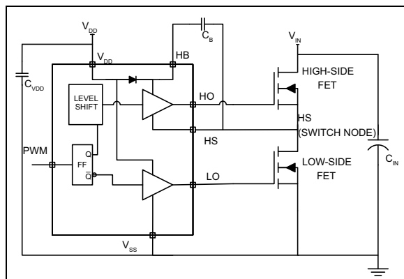
FIGURE 6-7: Typical Converter Power Stage.
