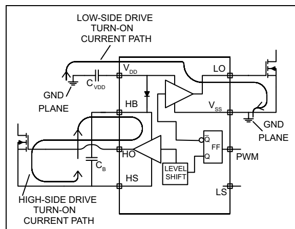
FIGURE 6-5: Turn-On Current Paths.
