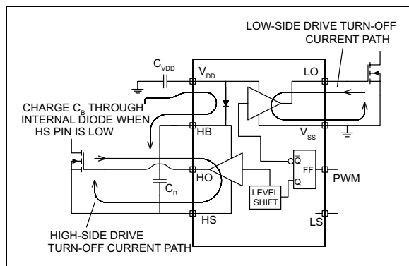
FIGURE 6-6: Turn-Off Current Paths.
