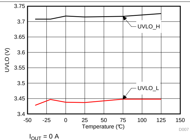
Figure 12. UVLO Threshold
