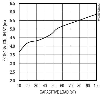
PROPAGATION DELAY vs. CAPACITIVE LOAD ON I/O V_L (DRIVING I/O V_{CC} = 3.3V , V_L = +0.9V )
