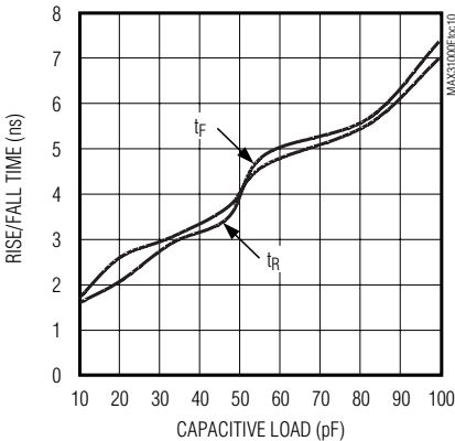
RISE/FALL TIME vs. CAPACITIVE LOAD ON I/O V_L (DRIVING I/O V_{CC} = 3.3V , V_L = +0.9V )
