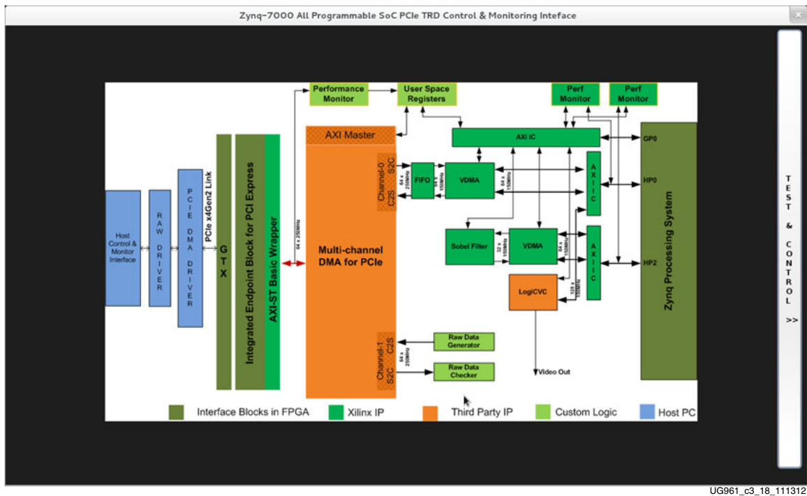
Figure 3-22: Design Block Diagram
