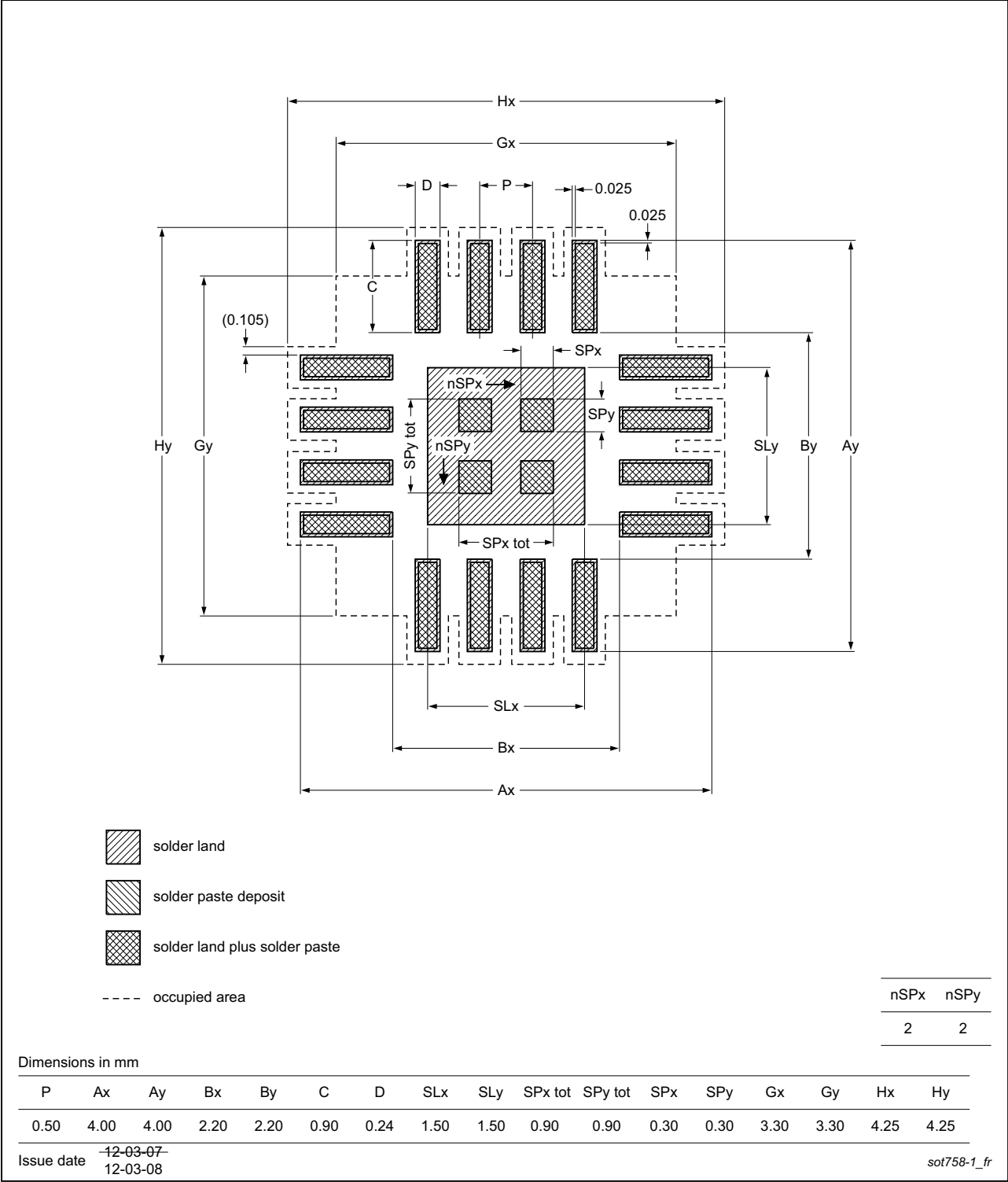
Fig 26. PCB footprint for SOT758-1 (HVQFN16); reflow soldering
