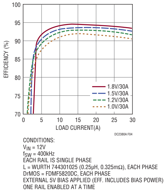
Figure 4. Efficiency Curves for the -A Converter at 12V_{IN}
