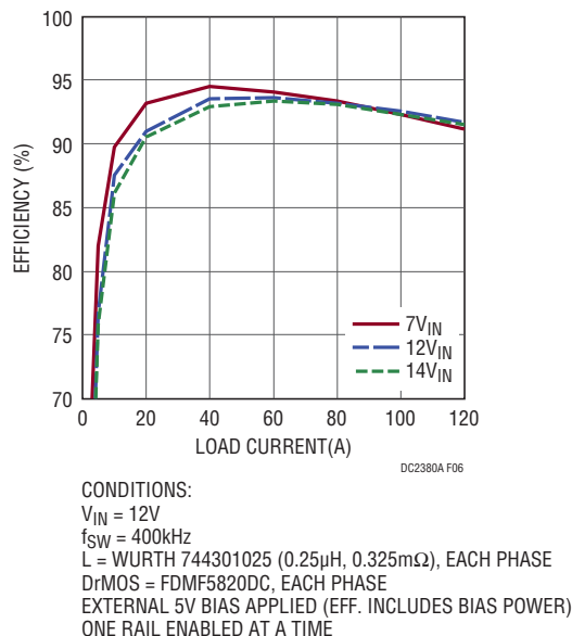
Figure 6. Efficiency Curves for the -C Converter Over the Input Voltage Range
