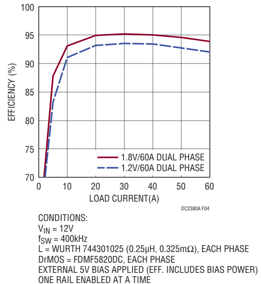
Figure 5. Efficiency Curves for the -B Converter at 12V_{IN}
