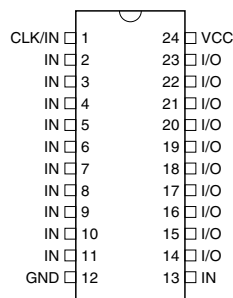
Figure 2-2. DIP/SOIC
