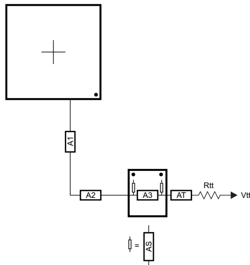
Figure 7-57. ADDR_CTRL Routing for Two Mirrored DDR3 Devices
