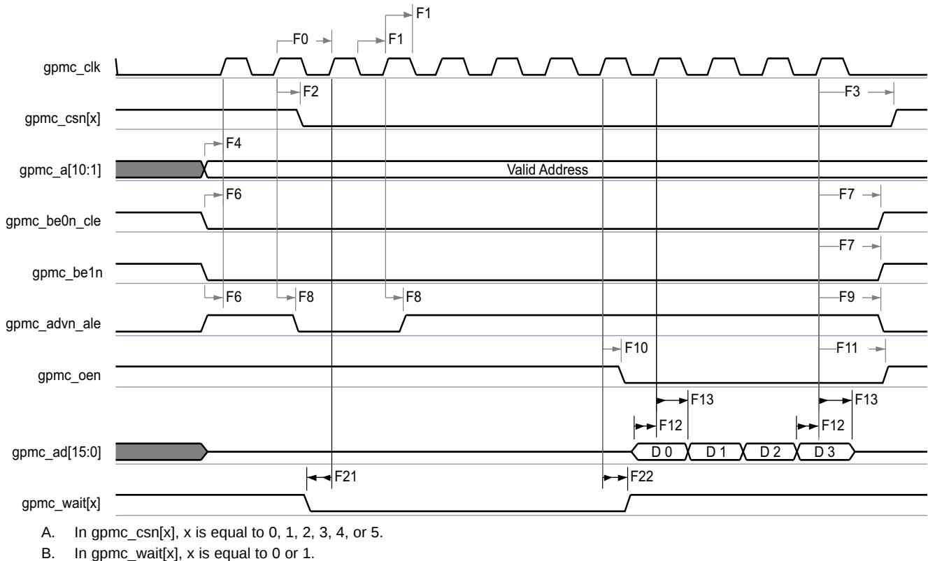
Figure 7-18. GPMC and NOR Flash—Synchronous Burst Read—4x16-Bit (GpmcFCLKDivider = 0)
