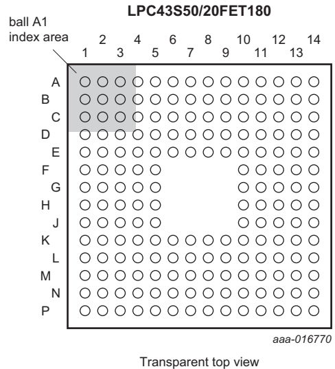
Fig 3. Pin configuration TFBGA180 package
