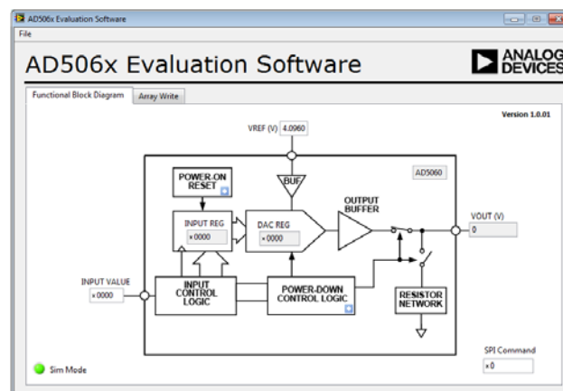
Figure 5. AD506x Evaluation Software Main Window
