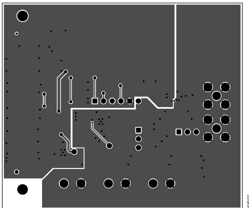
Figure 11. Printed Circuit Board, Solder Side
