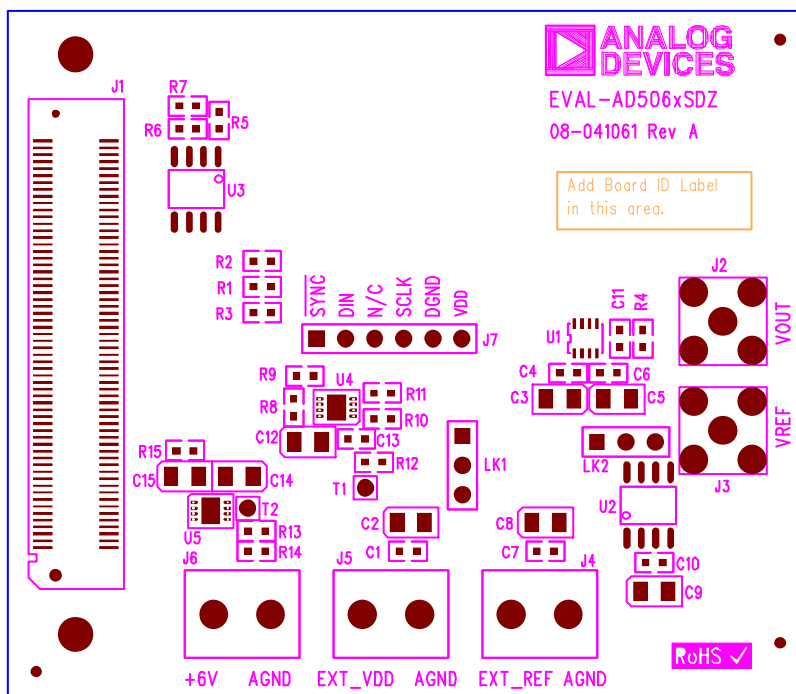
Figure 9. Component Placement Drawing
