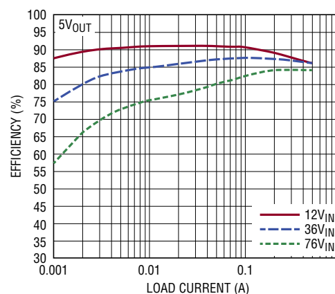
Figure 3. Efficiency Curves
