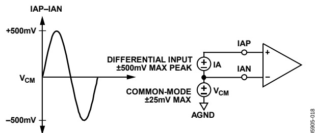
Figure 13. Maximum Signal Levels, Current Channel
