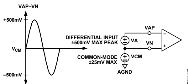
Figure 14. Maximum Signal Levels, Voltage Channel
