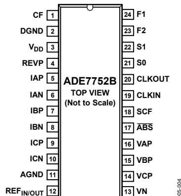
Figure 3. Pin Configuration
