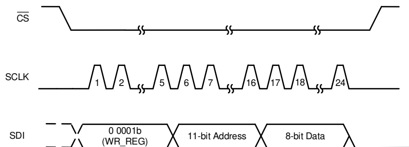
Figure 58. Register Write Operation
