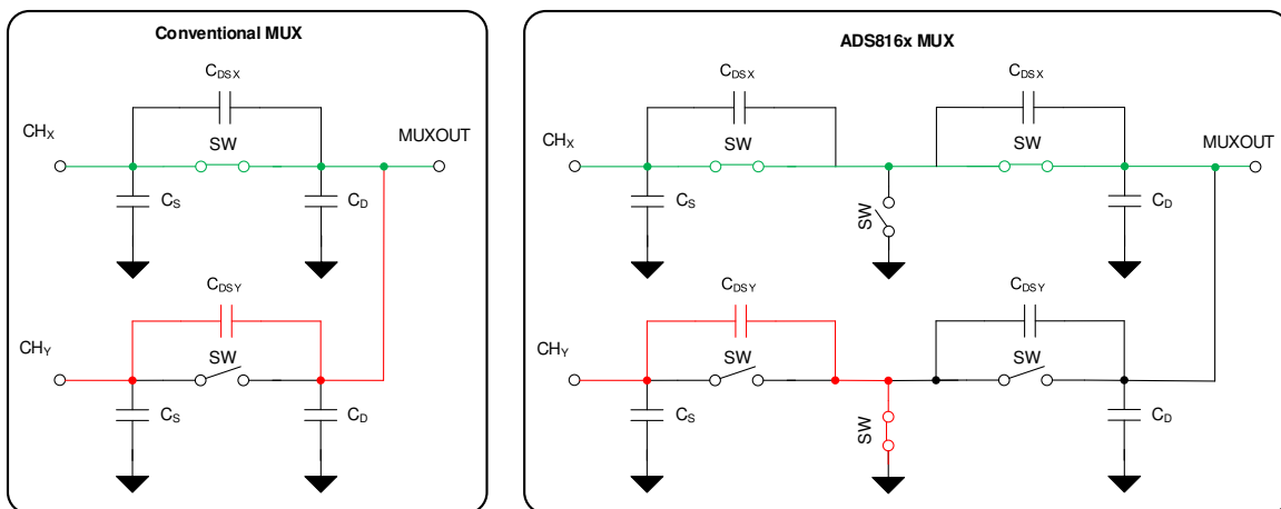
Figure 32. Isolation Crosstalk in a Conventional MUX versus the ADS816x
