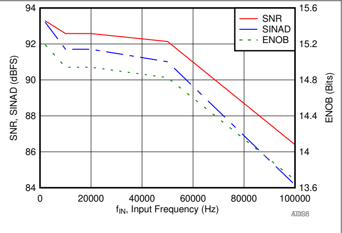
Figure 26. Noise Performance vs Input Frequency
