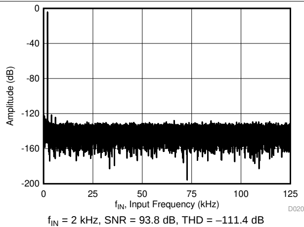
Figure 21. Typical FFT, ADS8166
