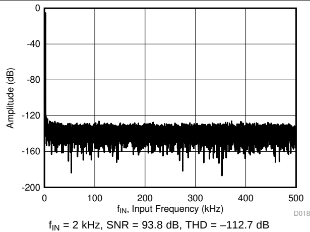
Figure 19. Typical FFT, ADS8168
