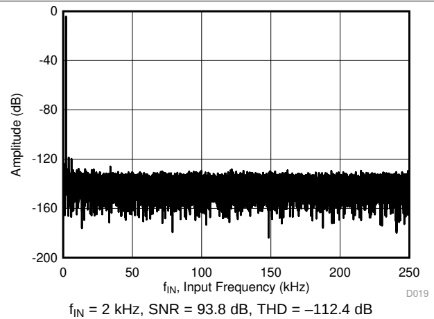
Figure 20. Typical FFT, ADS8167
