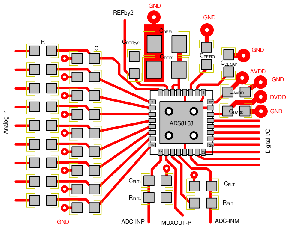
Figure 108. Recommended Layout
