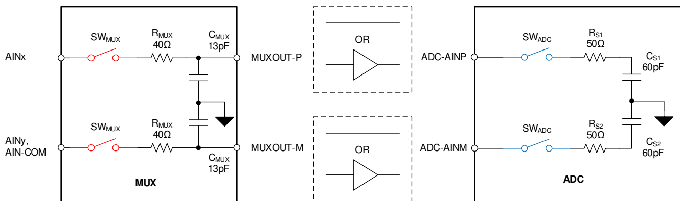
Figure 33. Synchronous and Timed Switching of the MUX and ADC Input Switches
