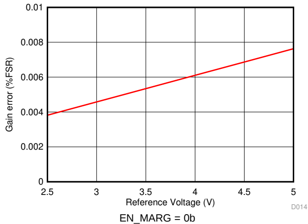
Figure 17. Gain Error (ADC + REFBUF) vs Reference Voltage
