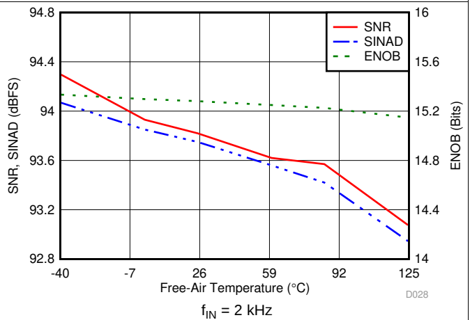
Figure 22. Noise Performance vs Temperature
