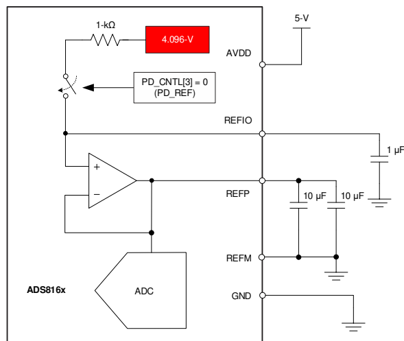
Figure 35. Device Connections for Using an Internal 4.096-V Reference
