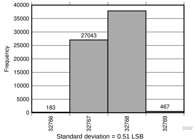
Figure 18. DC Input Histogram
