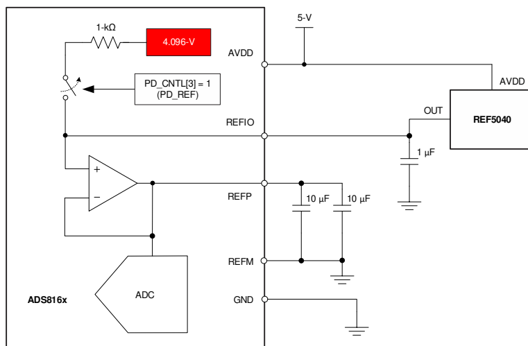
Figure 36. Device Connections for Using an External Reference
