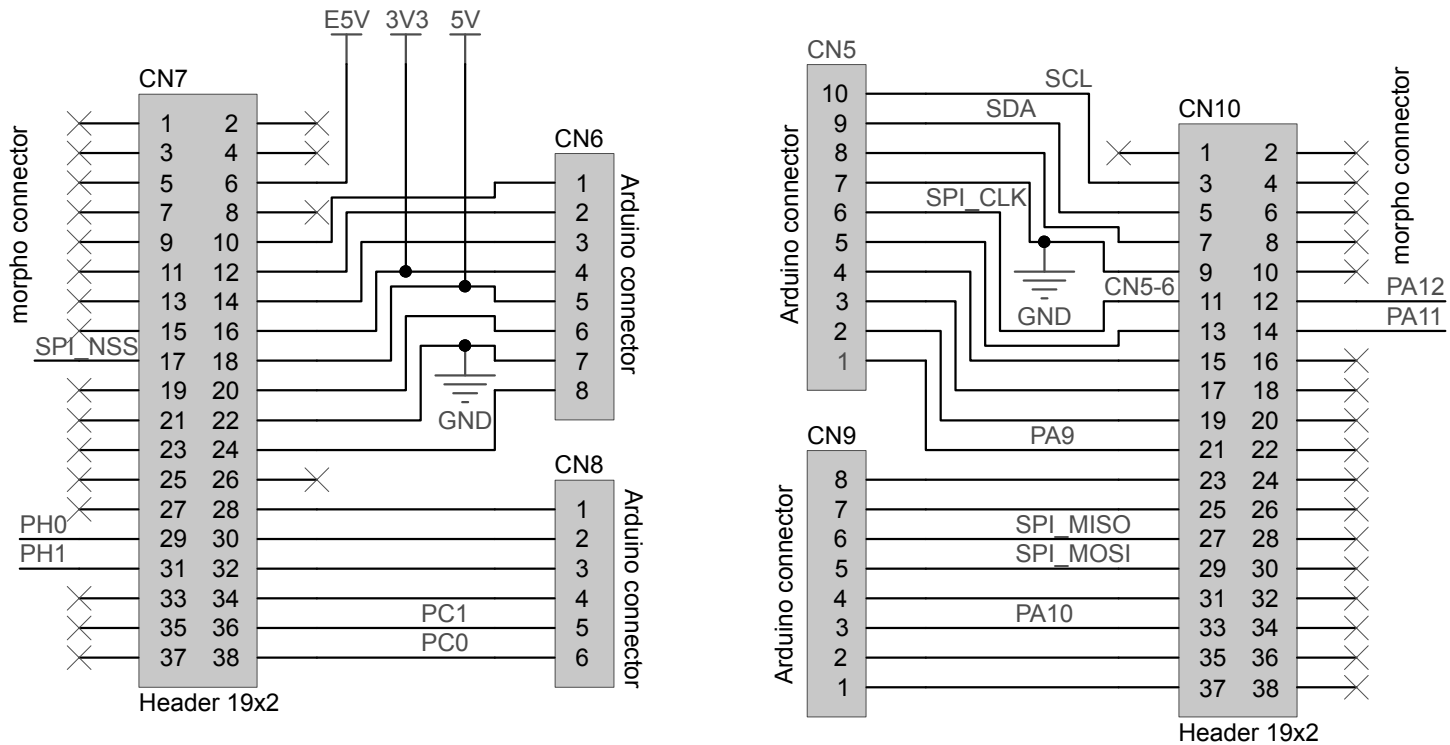
Figure 3. X-NUCLEO-SAFEA1 circuit schematic - Arduino and morpho connectors
