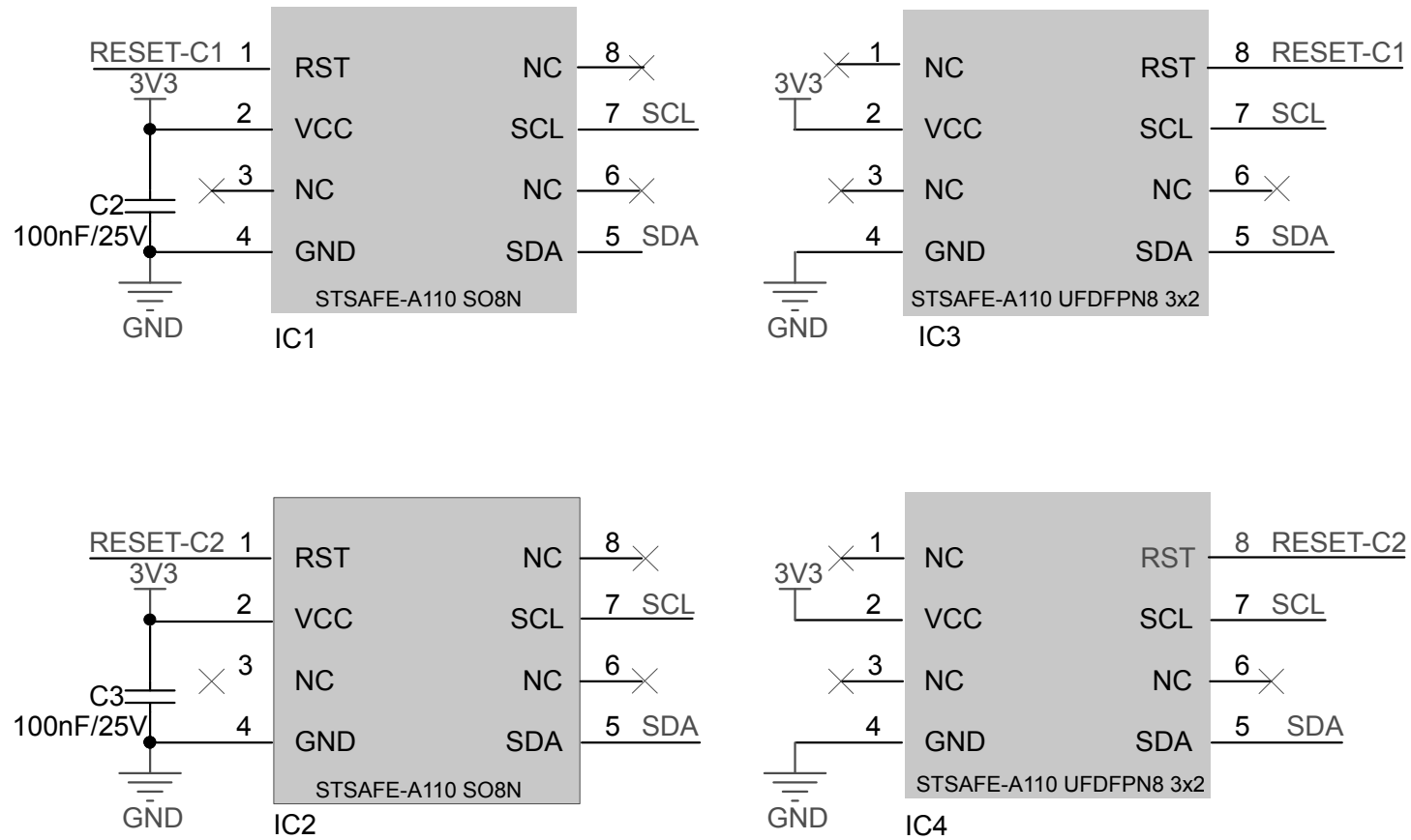
Figure 2. X-NUCLEO-SAFE1 circuit schematic - STSAFE-A chips
