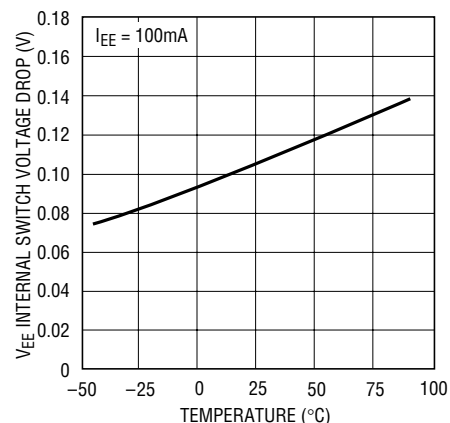
V_{EE} Internal Switch Voltage Drop vs Temperature
