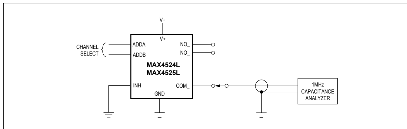
Figure 5. NO/COM Capacitance
