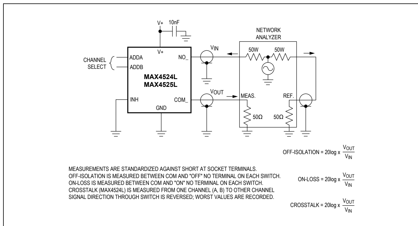
Figure 6. Off-Isolation, On-Loss, and Crosstalk
