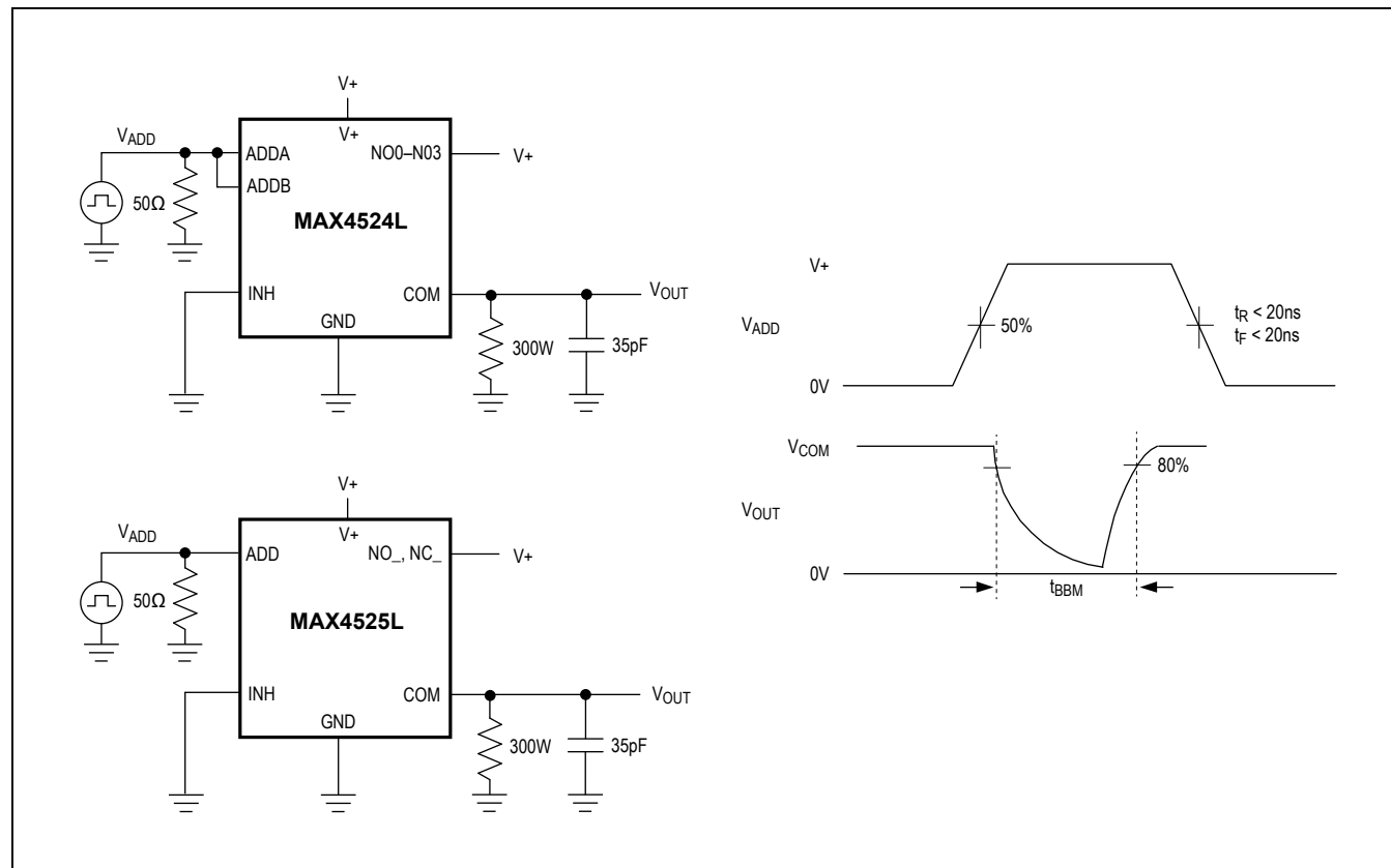
Figure 3. Break-Before-Make Interval
