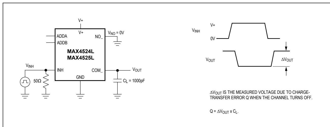
Figure 4. Charge Injection
