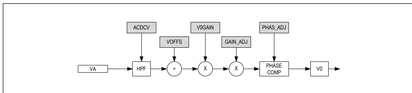
Figure 5. Voltage Signal Data Path
