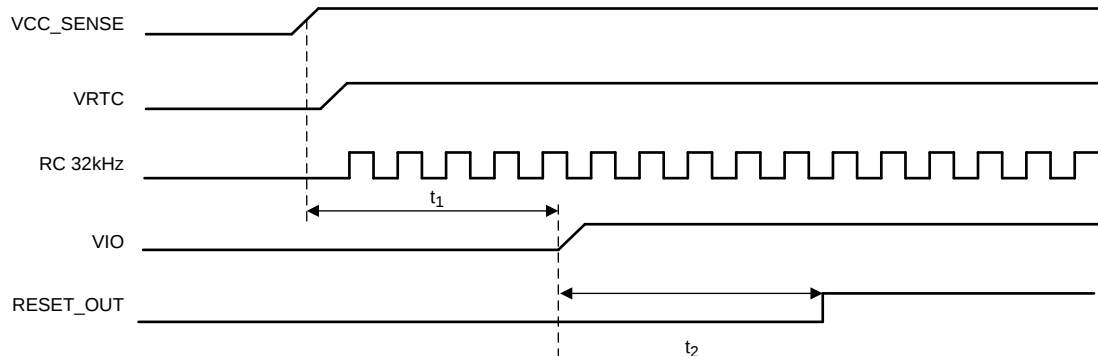
Figure 5-4. TPS65917-Q1 Power-Up Sequence After FSD
