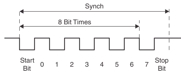
Figure 10-6. Auto Baud-Rate Detection – Synch Field
