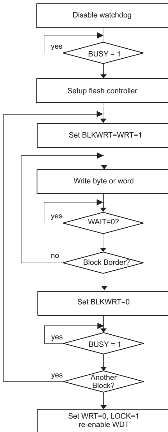
Figure 5-11. Block Write Flow
