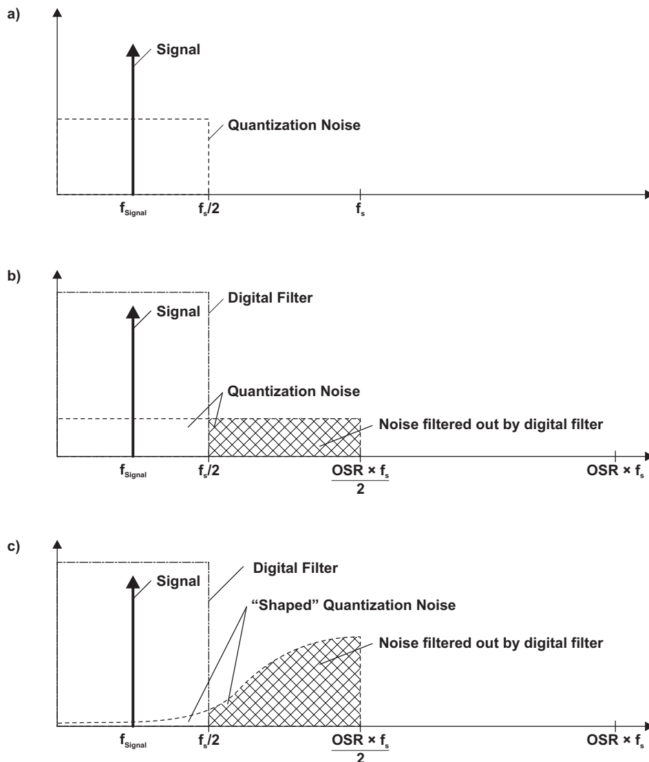
Figure 13-2. Sigma-Delta Principle
