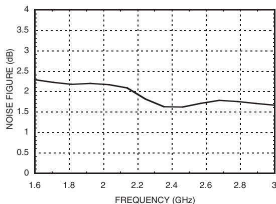
Broadband Noise Figure
