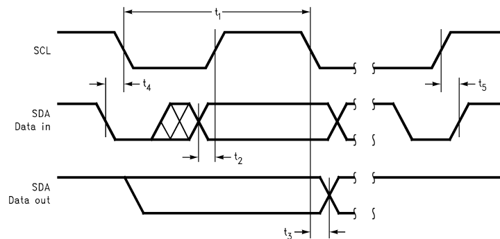
Figure 54. I²C Timing Diagram
