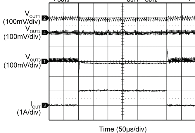
Transient Cross Regulation ( I_{OUT3} = 20\text{mA} to 1A; I_{OUT1}, I_{OUT2} = 20\text{mA} )
