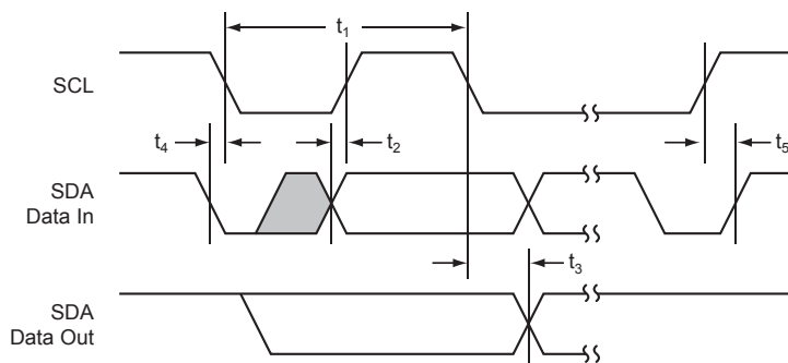
Figure 1. SMBus Timing
