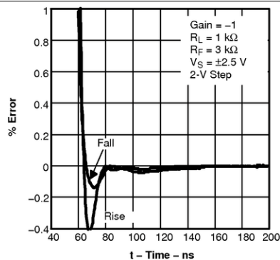
Figure 34. Settling Time
