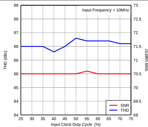
Figure 87. Performance vs Input Clock Duty Cycle
