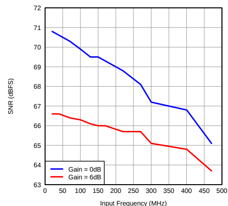
Figure 93. SNR vs Input Frequency (CMOS)
