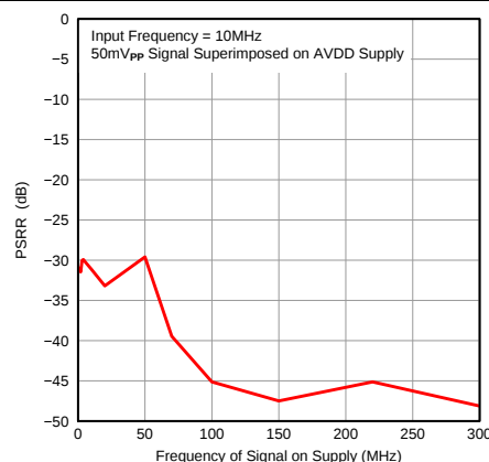
Figure 125. PSRR vs Test Signal Frequency
