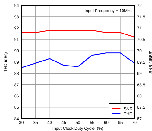
Figure 123. Performance vs Input Clock Duty Cycle
