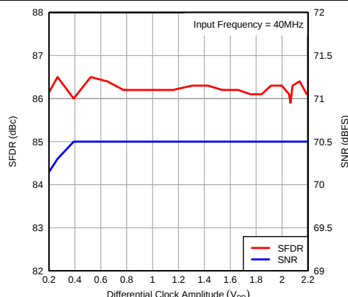
Figure 85. Performance vs Input Clock Amplitude
