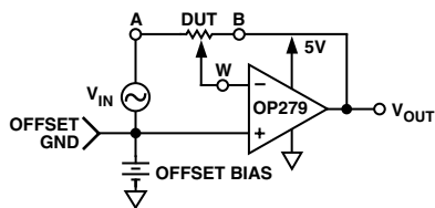
Figure 10. Inverting Gain Test Circuit
