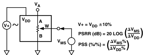
Figure 9. Power Supply Sensitivity Test Circuit (PSS, PSRR)
