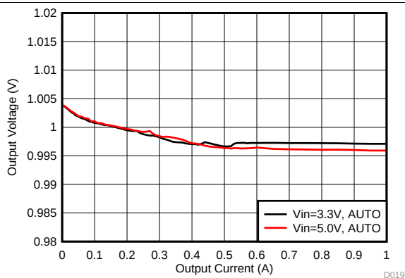
Figure 30. Buck Output Voltage vs Load Current in PFM/PWM Mode
