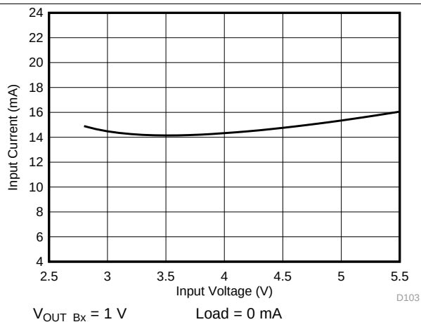
Figure 4. Active State Current Consumption vs Input Voltage, One Buck Regulator Enabled in Forced PWM Mode
