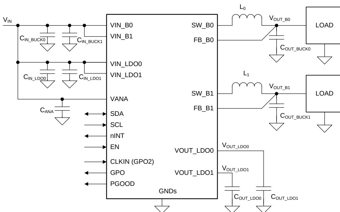
Figure 25. LP87322B/D/E/F-Q1 Typical Application
