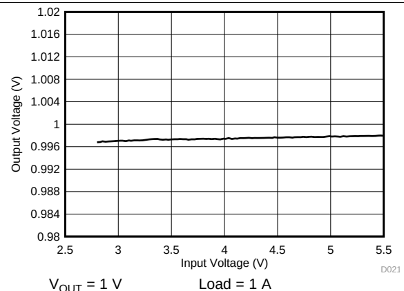
Figure 31. Buck Output Voltage vs Input Voltage in PWM Mode
