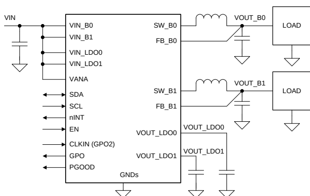
Simplified Schematic
