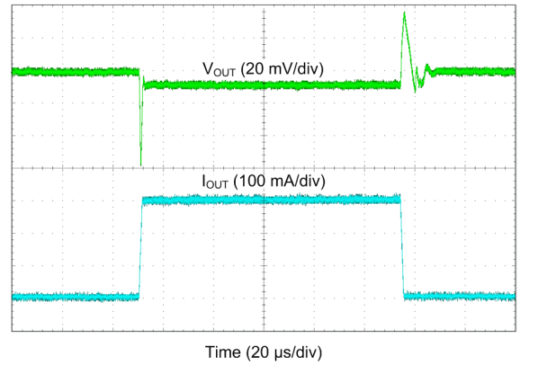
Figure 51. LDO Transient Load Step Response
