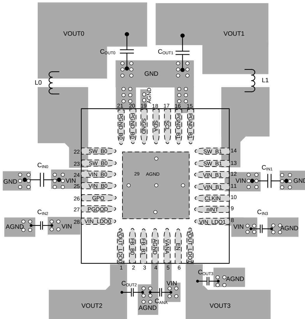
Figure 55. LP87322B/D/E/F-Q1 Board Layout
