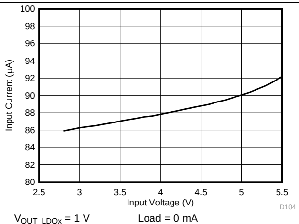
Figure 5. Active State Current Consumption vs Input Voltage, One LDO Regulator Enabled
