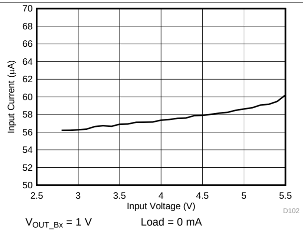
Figure 3. Active State Current Consumption vs Input Voltage, One Buck Regulator Enabled in PFM Mode
