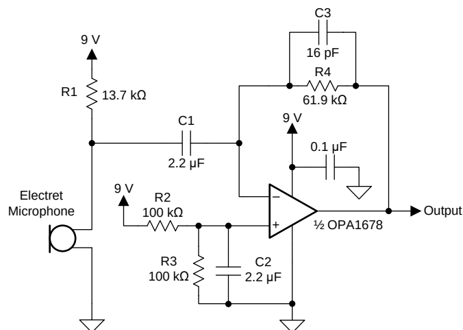
Figure 39. Single-Supply Electret Microphone Preamplifier
