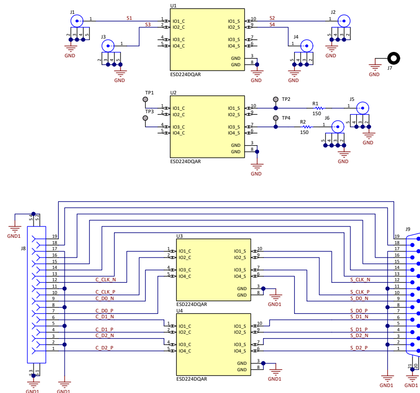
Figure 6. ESD224EVM Schematic
