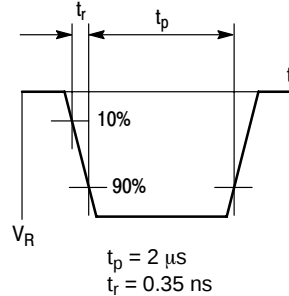
INPUT PULSE
