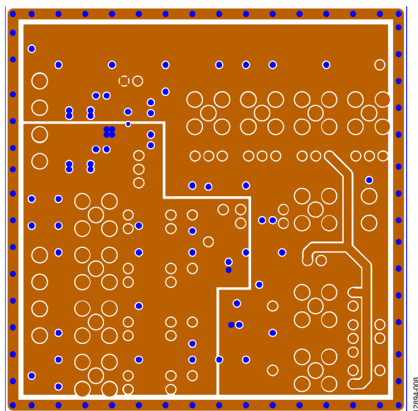
Figure 8. EVAL-ADG5404FEBZ Layer 3
