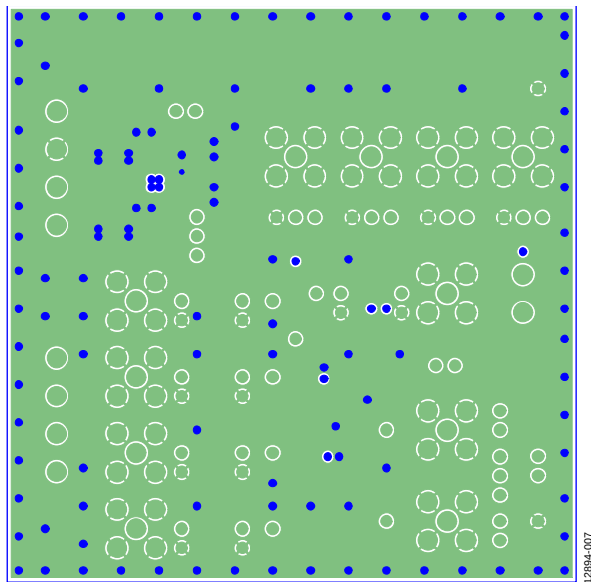
Figure 7. EVAL-ADG5404FEBZ Layer 2
