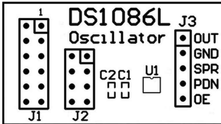
Figure 2. DS1086LPMB11 Peripheral Module Component Placement Guide—Component Side
