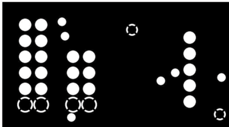
Figure 4. DS1086LPMB11 Peripheral Module PCB Layout—Inner Layer 1 (Ground)
