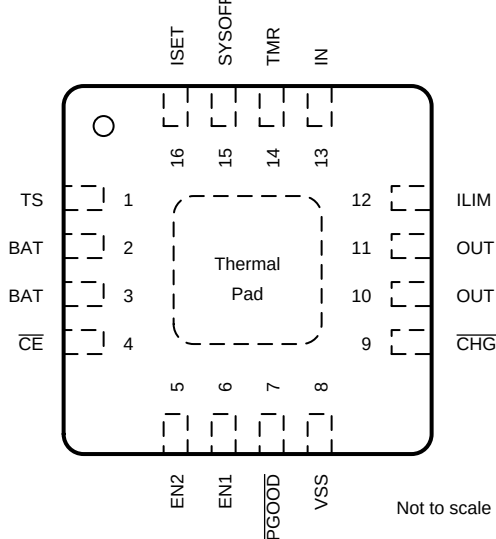
BQ24075 RGT0016C Package, BQ24079 RGT0016B Package 16 Pins Top View
