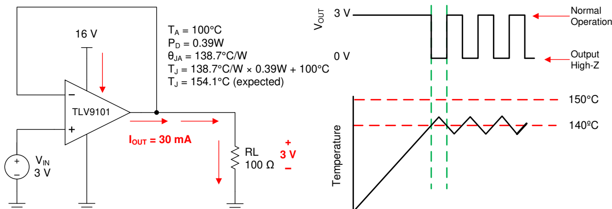
Figure 46. Thermal Protection
