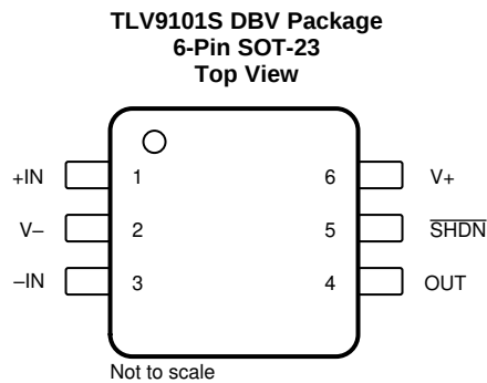
Pin Functions: TLV9101S
