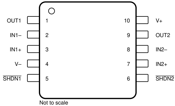
TLV9102S DGS Package 10-Pin VSSOP Top View
