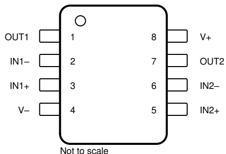
TLV9102 D, DDF, DGK, and PW Package (1) 8-Pin SOIC, SOT-23, TSSOP, and VSSOP Top View
