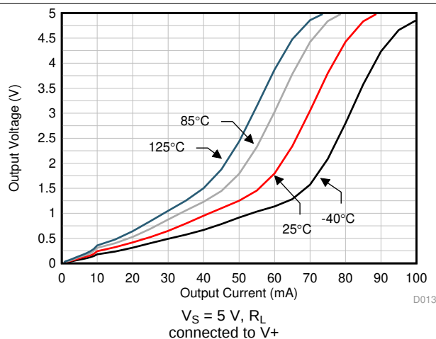
Figure 17. Output Voltage Swing vs Output Current (Sinking)
