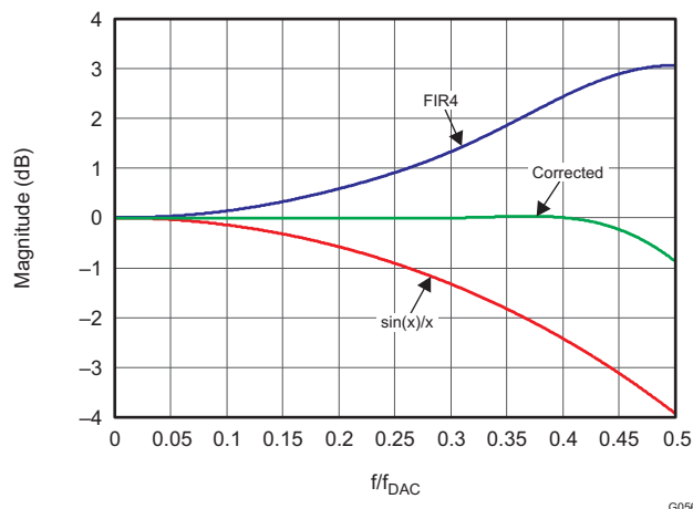
Figure 43. Composite Magnitude Spectrum for INVSINC
