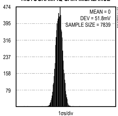
HISTOGRAM: IQ GAIN IMBALANCE
