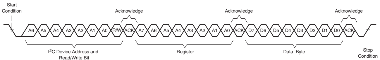
Figure 89. I²C Single-Byte Write Transfer
