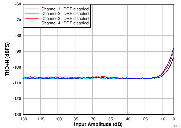
Figure 8. THD+N vs Input Amplitude With DRE Disabled
