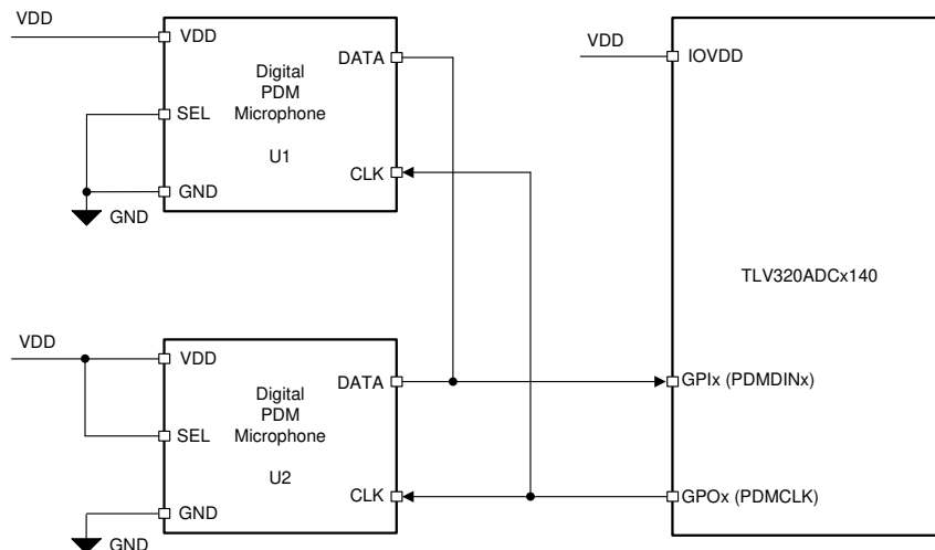
Figure 86. Digital PDM Microphones Connection Diagram to the TLV320ADC6140
