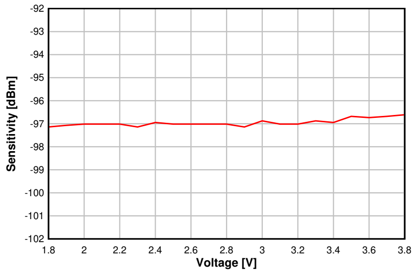
Figure 5-15. Sensitivity vs. Supply Voltage (VDDS) (BLE 1 Mbps, 2.44 GHz)
