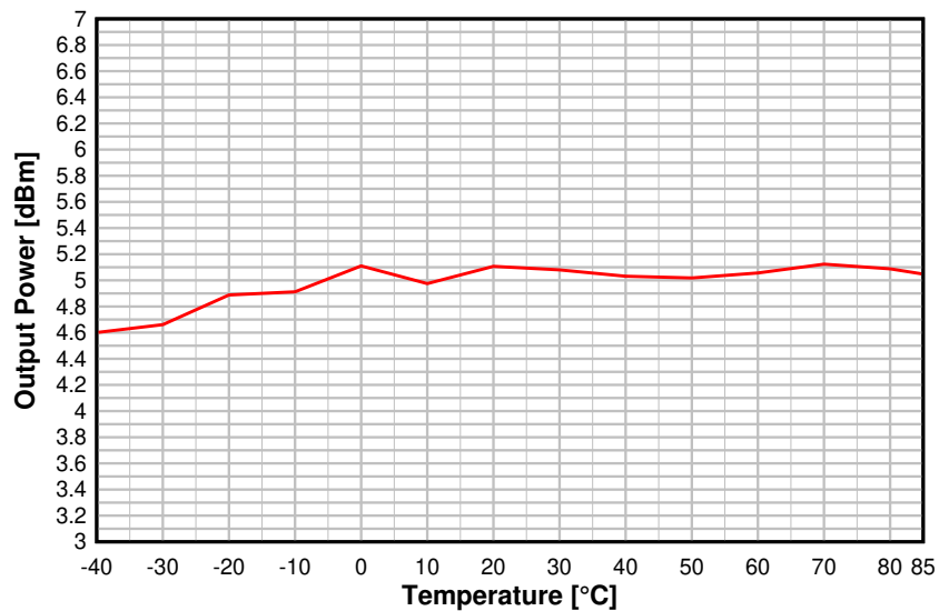
Output Power vs. Temperature BLE 1 Mbps, 2.44 GHz, +5 dBm
