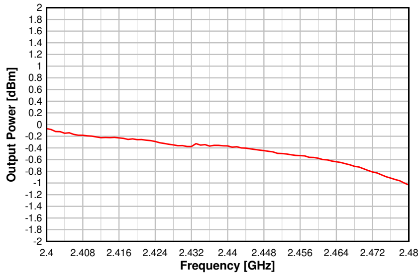
Figure 5-22. Output Power vs. Frequency (BLE 1 Mbps, 2.44 GHz, 0 dBm)
