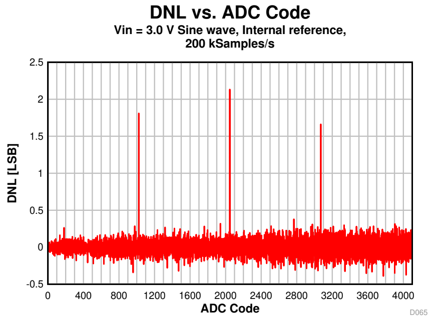
Figure 5-28. DNL vs. ADC Code
