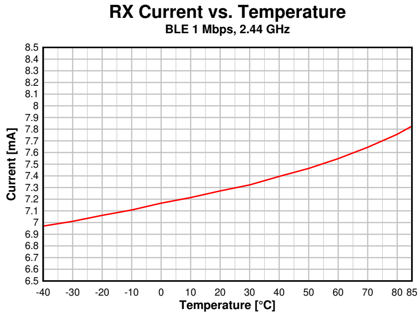
Figure 5-7. RX Current vs. Temperature (BLE 1 Mbps, 2.44 GHz)
