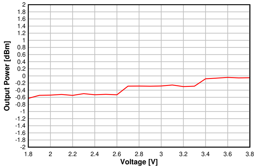
Figure 5-20. Output Power vs. Supply Voltage (VDD5) (BLE 1 Mbps, 2.44 GHz, 0 dBm)
