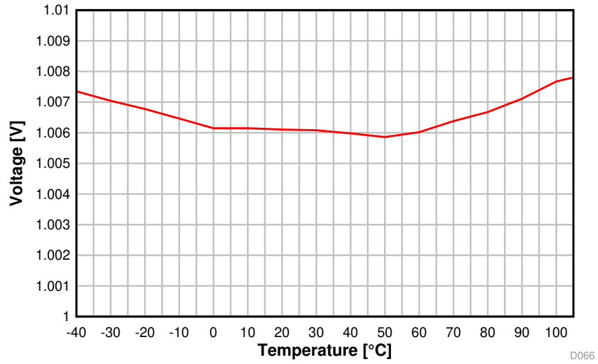
Figure 5-29. ADC Accuracy vs. Temperature
