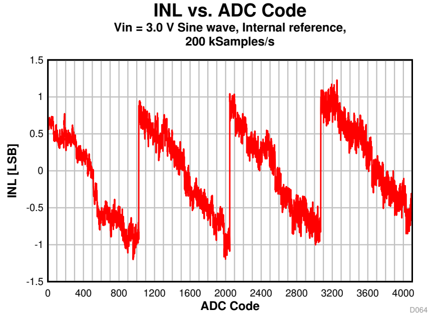
Figure 5-27. INL vs. ADC Code
