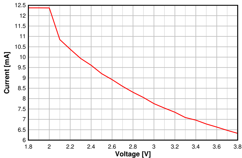
TX Current vs. VDD5 BLE 1 Mbps, 2.44 GHz, 0 dBm
