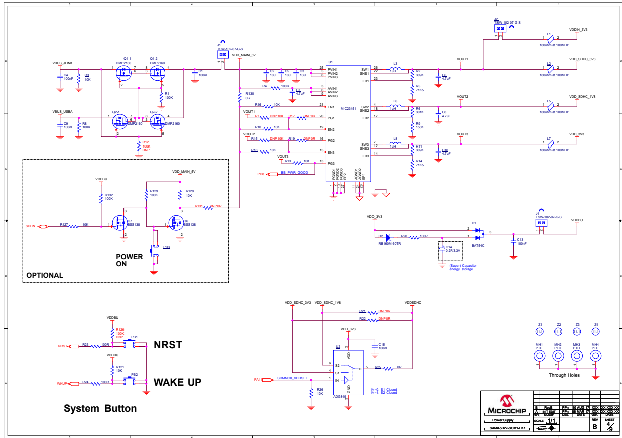
Figure 7-4. Power Supply
