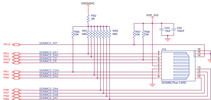
Figure 4-14. SDMMC0
