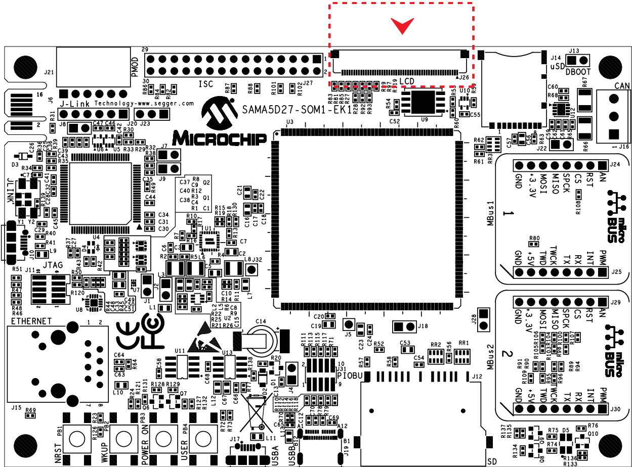
Figure 4-30. LCD Connector J26 Location
