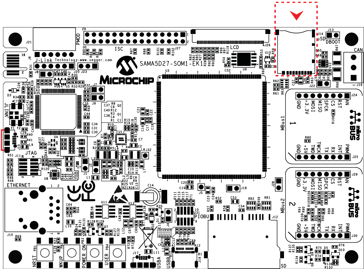
Figure 4-17. microSD Socket J14 Location
