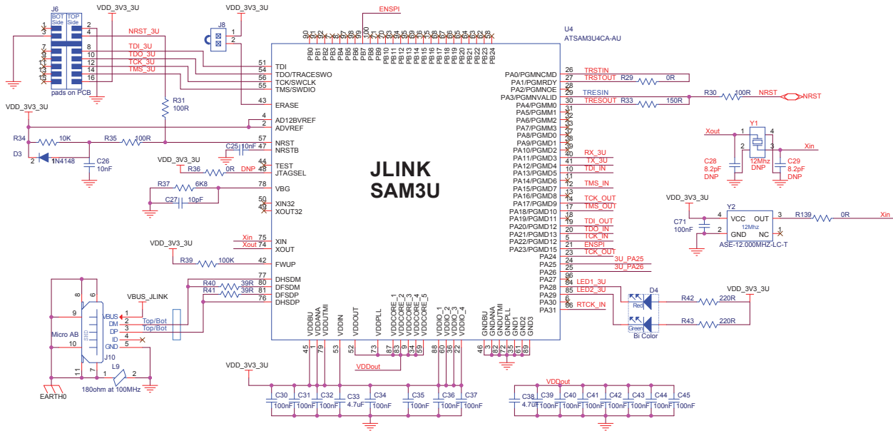
Figure 4-36. J-Link-OB Interface
