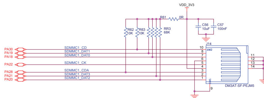
Figure 4-16. SDMMC1 microSD
